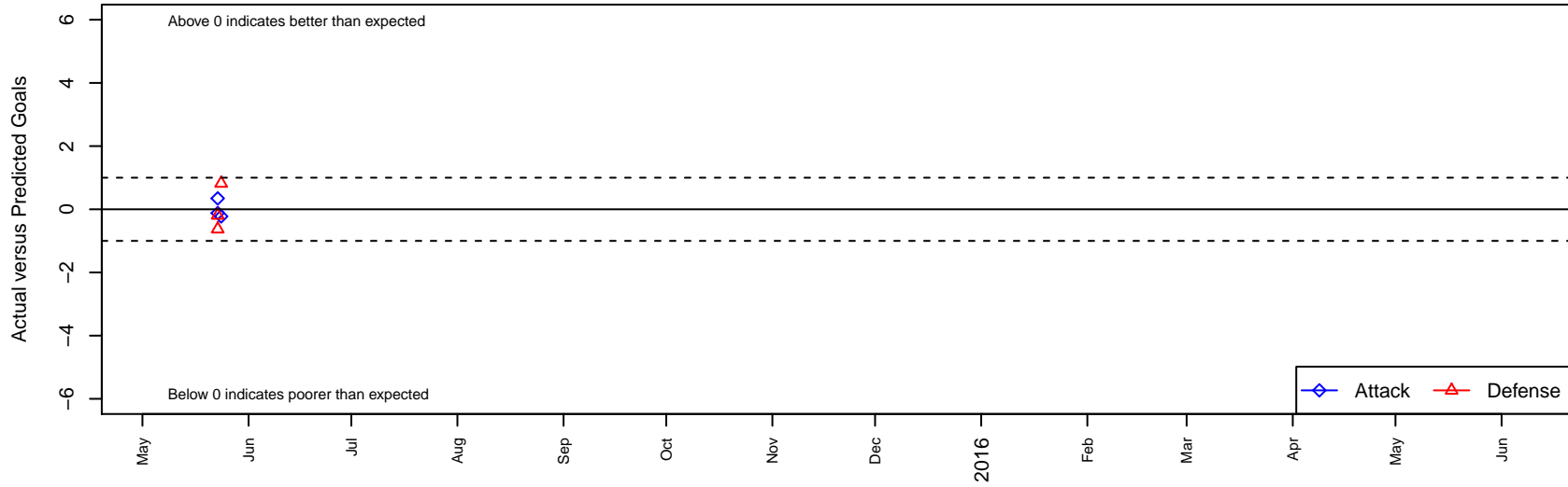
San Francisco United Barcelona Red B00 Dots are actual minus expected GF (blue circles) and GA (red triangles). Blue line is smoothed change in attack strength. Red is smoothed change in defense strength.
